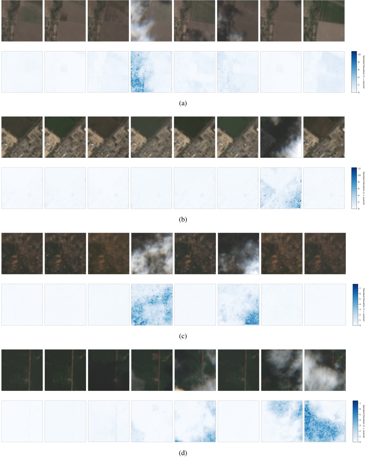
Figure 10: Visualization of estimated uncertainty maps. Four examples from the WorldStrat-bitter dataset, each showing LR frames (top row) and the corresponding estimated uncertainty maps (bottom row). The uncertainty maps highlight cloudy or inconsistent pixels, enabling the GNLL loss to downweight these during optimization.
