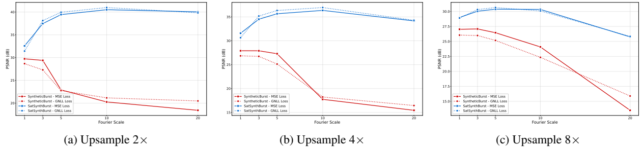
Figure 7: Sensitivity analysis of the Fourier feature scale. The optimal hyperparameter depends on the domain, i.e. satellite imagery (SatSynthBurst in blue) and ground-level bursts (SyntheticBurst in red) require different settings. However, the optimal setting is invariant to the loss. For SyntheticBurst we see a small difference between the upsampling factor experiments. However, we note that the two datasets differ in the strategy of creating different upsampling factors. The SyntheticBurst varies the HR output resolution with a fixed resolution of the LR frames. Hence, the absolute output resolution may affect the optimal Fourier feature scale. In contrast, the SatSynthBurst dataset fixes the HR output resolution and varies the resolution of the LR frames.
