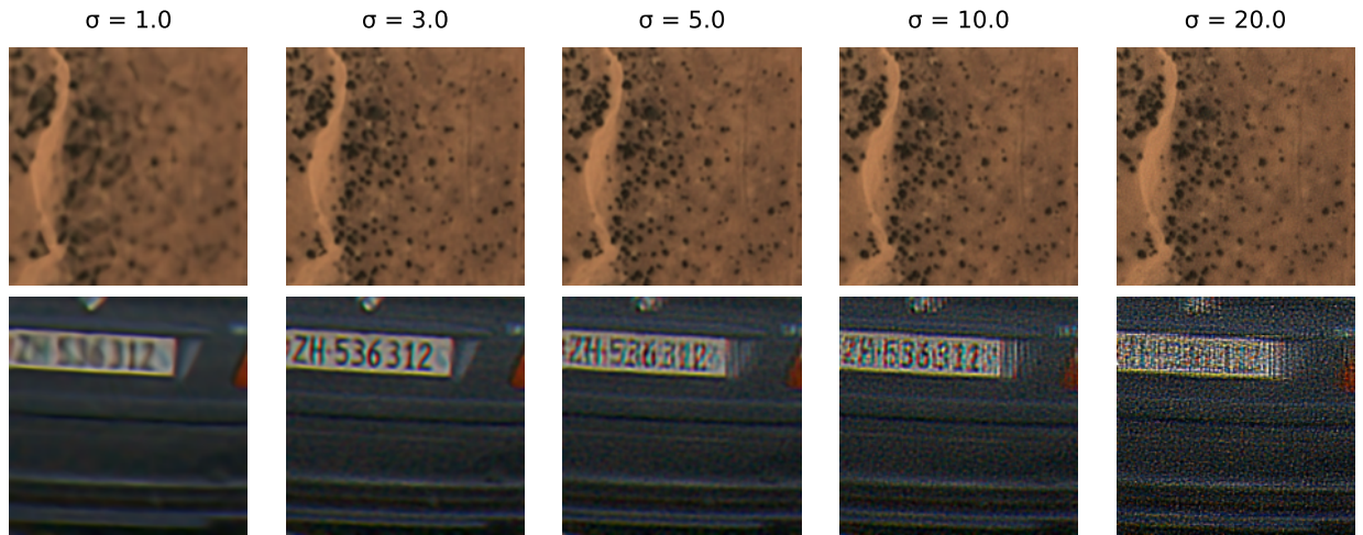
Figure 8: Effect of the Fourier feature scale \sigma for MSE (upsampling factor \times 4 ). The optimal hyperparameter depends on the domain, i.e. satellite imagery and ground-level bursts require different settings. Setting the scale too low leads to over-smoothing, whereas setting it too high leads to grainy artifacts.
