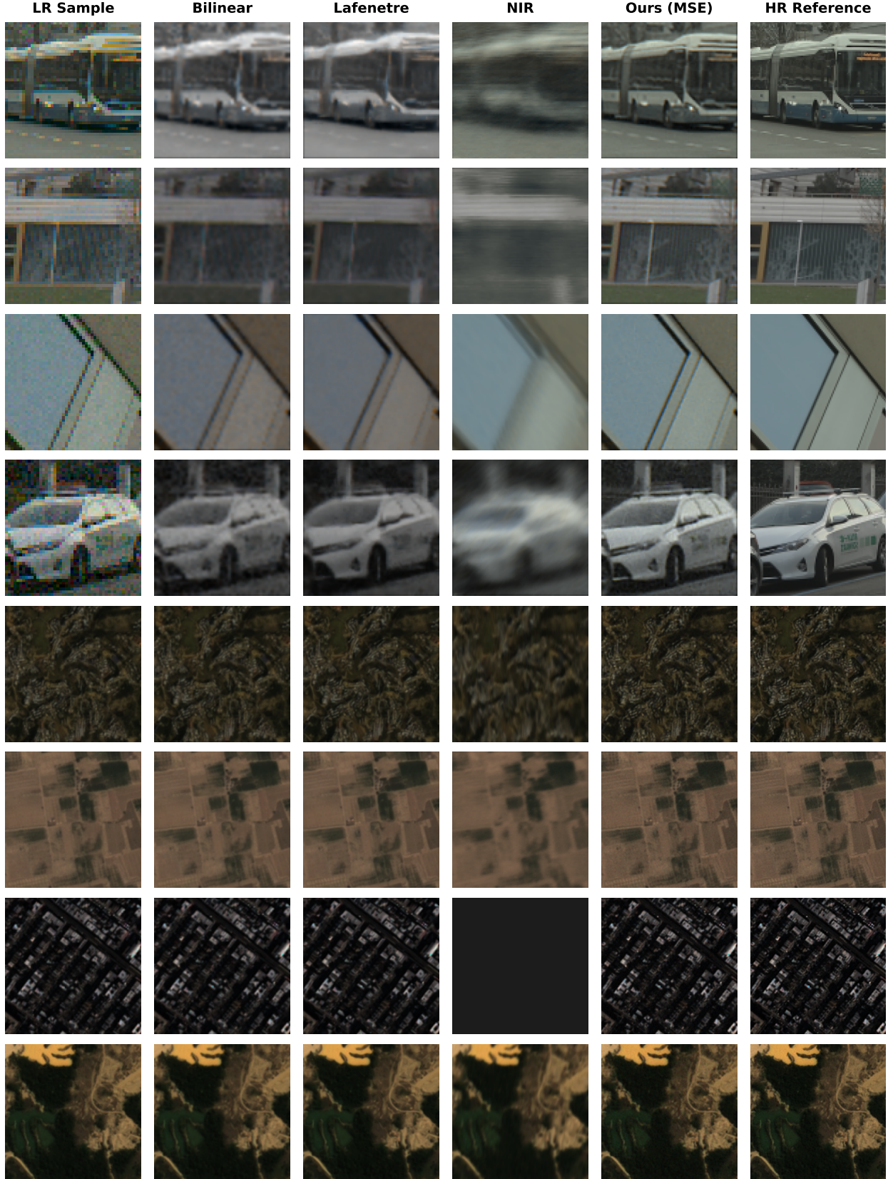
Figure 11: Qualitative comparison with upsampling factor \times 2 . From left to right, we show: one low-resolution (LR) frame, bilinear upsampling, steerable kernel regression (Lafetnetre et al., 2023), NIR (Nam et al., 2022), our SuperF approach, and the high-resolution (HR) reference.
