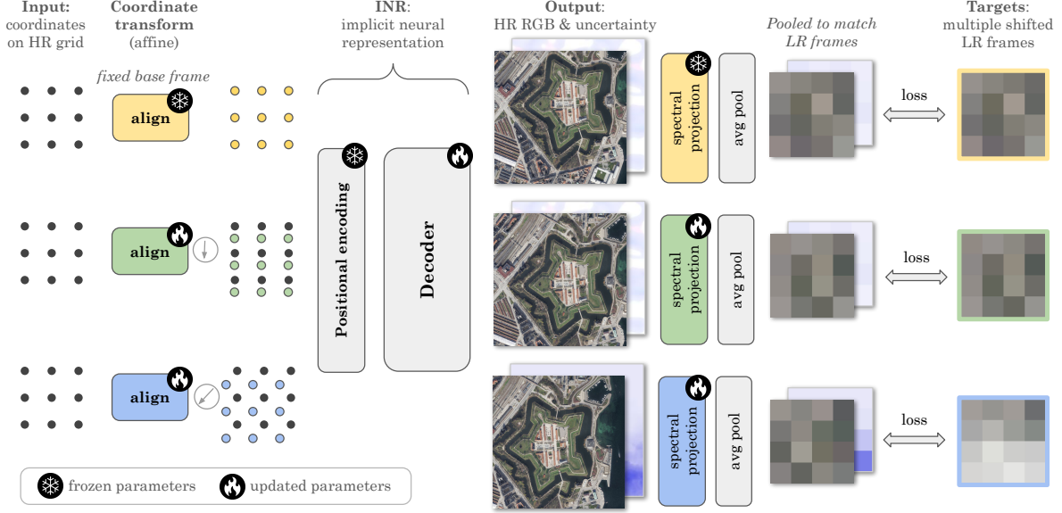
Figure 1: Illustration of the proposed method. SuperF achieves multi-image super-resolution by sharing an implicit neural representation (INR) across multiple low-resolution (LR) frames with sub-pixel shifts. The LR frames are aligned by jointly optimizing an affine coordinate transformation for each LR frame, together with the parameters of a coordinate-based multi-layer perceptron (MLP) that decodes the input coordinates to RGB values. Hence, leveraging the continuous characteristics of INRs for both the sub-pixel alignment in the pixel coordinate space and for representing the underlying high-resolution (HR) signal. For robustness, the proposed INR can optionally represent additional frame-specific uncertainty maps to ignore noisy pixels (e.g. clouds) in the optimization.
